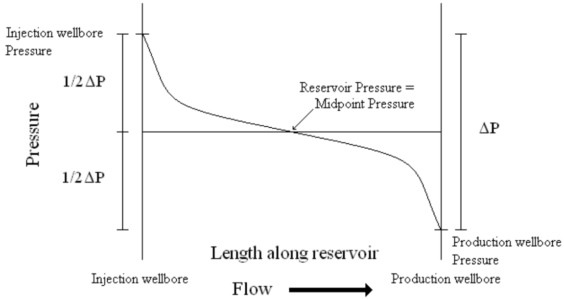
Figure 2 Reservoir pressure profile assumption expressed pictorially.
