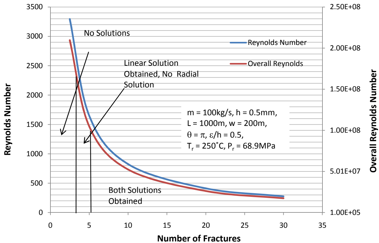
Figure 7 Reynolds number and overall Reynolds number versus number of fractures.
