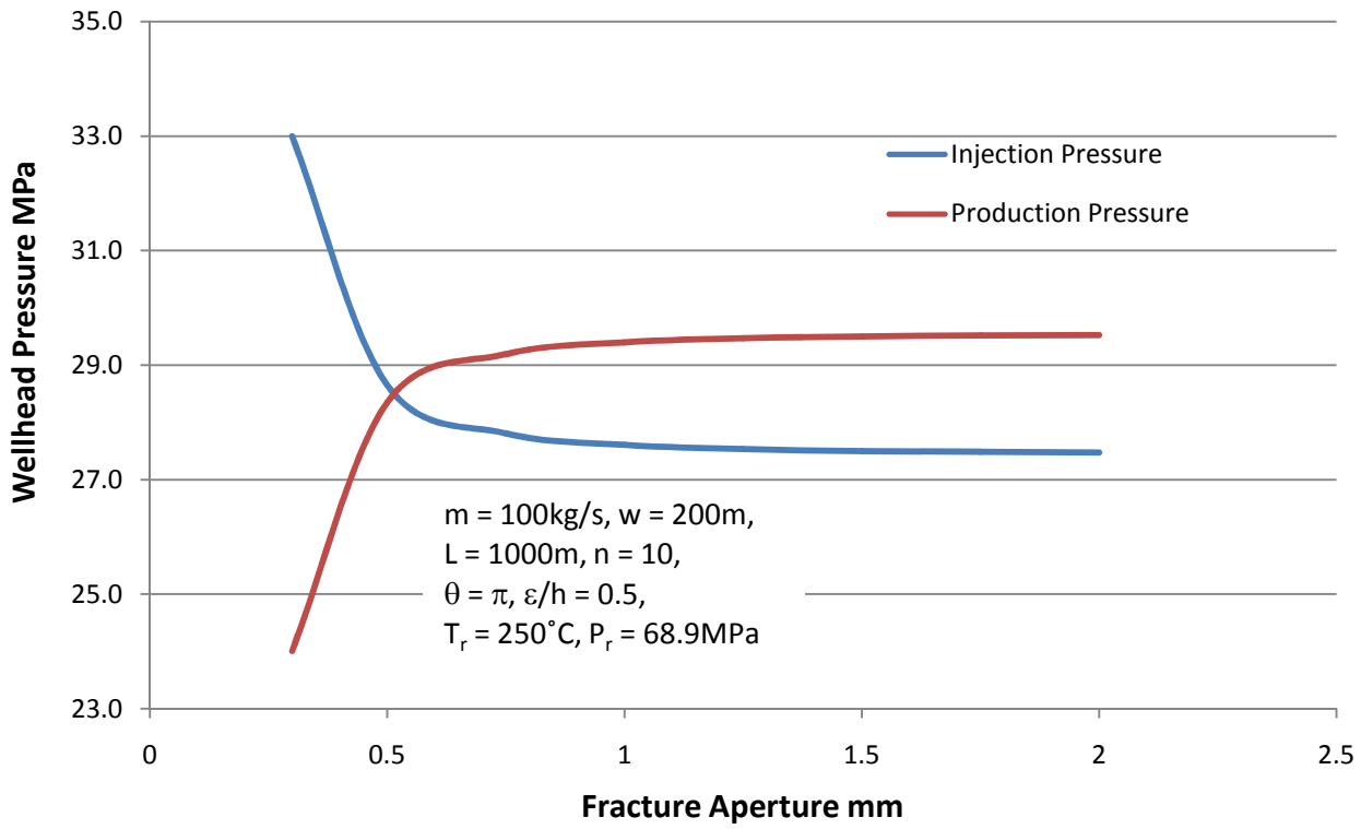
Figure 4 Wellhead injection and production pressure versus fracture aperture.
