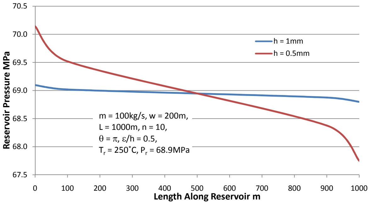
Figure 6 Reservoir pressure profile for fracture aperture 1mm and 0.5mm.
