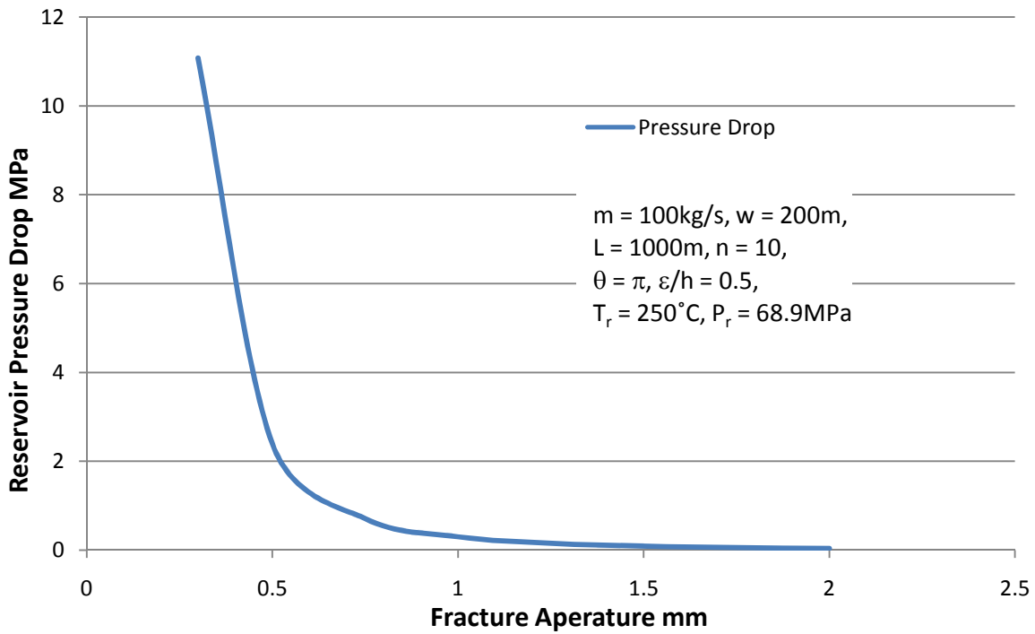
Figure 5 Reservoir pressure drop versus fracture aperture.
