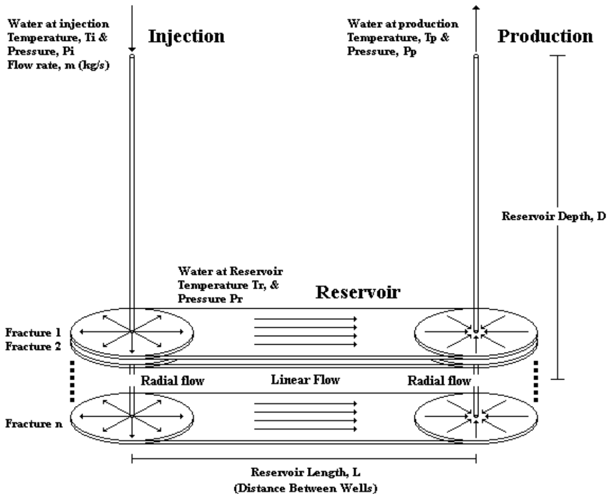
Figure 1 Geometry of EGS model.
