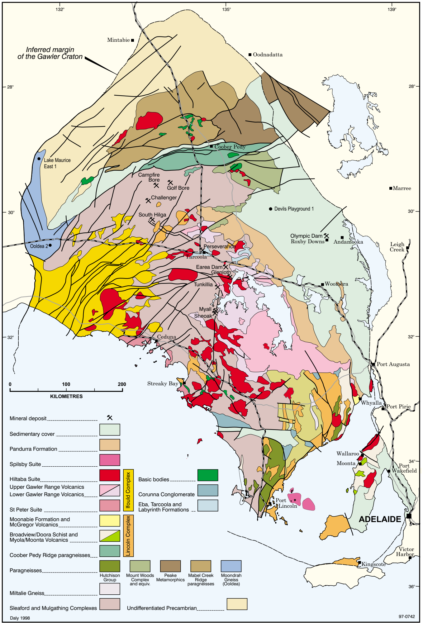
Interpreted subsurface geology of the Gawler Craton, South Australia
