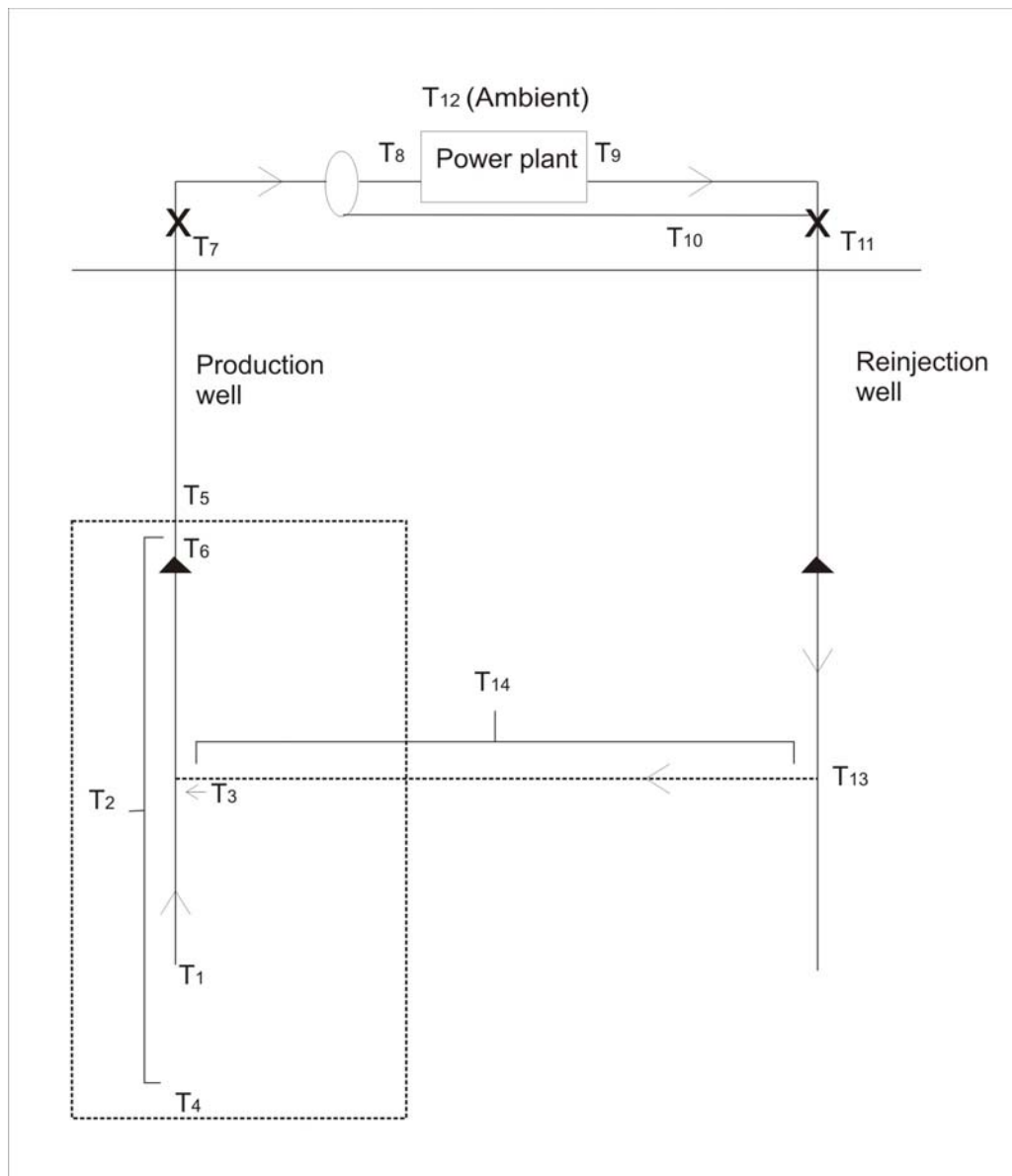
Figure A.1 Possible points for temperature definition within a production - reinjection well doublet and power scheme.
