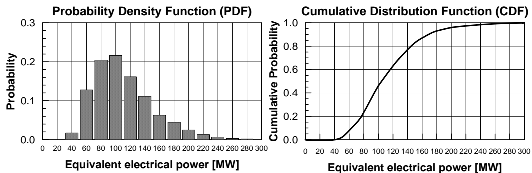
Figure 3: Monte Carlo Simulation Results
