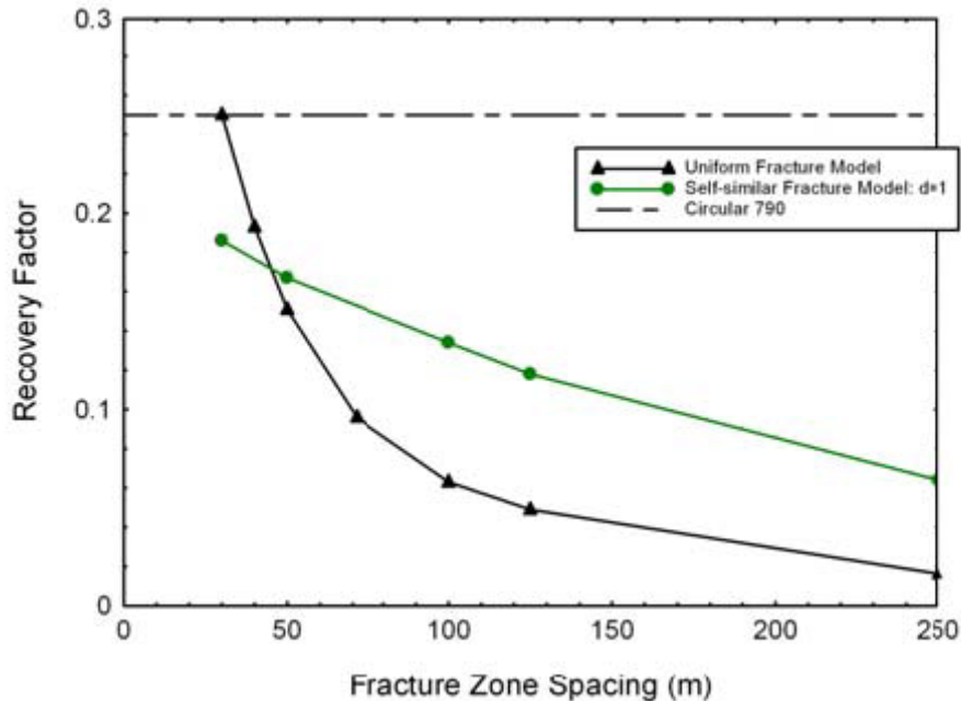
Figure 4: Variations in recovery factor with fracture spacing for example models incorporating planar fractures with uniform flow properties (black) and a fractal distribution of flow properties among the producing fractures (green).
