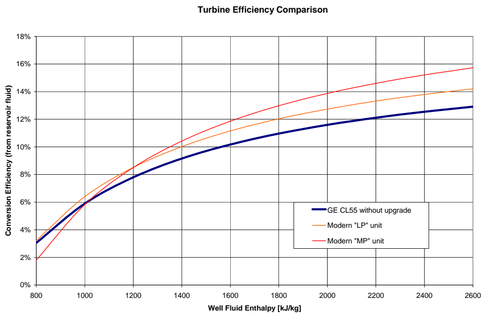
Figure 5; Typical efficiency for modern single flash condensing steam turbines and older marine surplus turbines such as have been used in geothermal applications. Higher efficiencies are achievable for the latter with some modifications. Note that the efficiency in this case is based on the energy content of the whole of the fluid abstracted from the wells, including the separated water which is not made use of.
