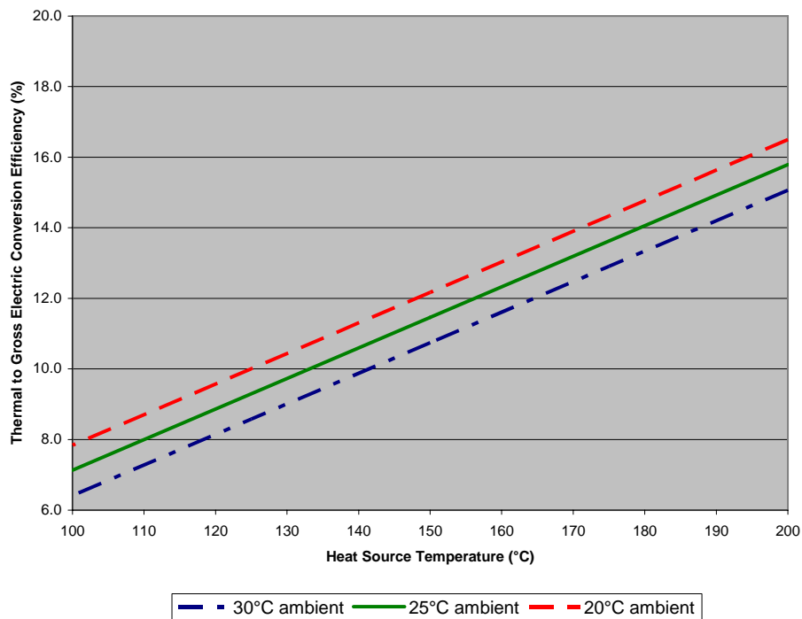
Figure 6; Typical efficiency for ORC binary plant, at a range of ambient temperatures and assuming single phase liquid input Note that the efficiency in this case is gross electricity output: typically binary plant would consume 10 to 20% of gross power in-house, excluding any reinjection pumping.
