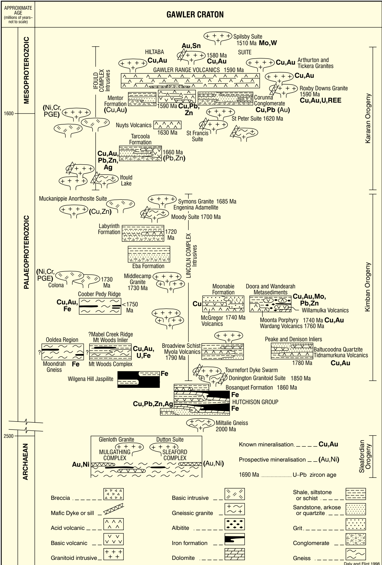
Nomenclature and suggested correlation of Precambrian rock units in the Gawler Craton.
